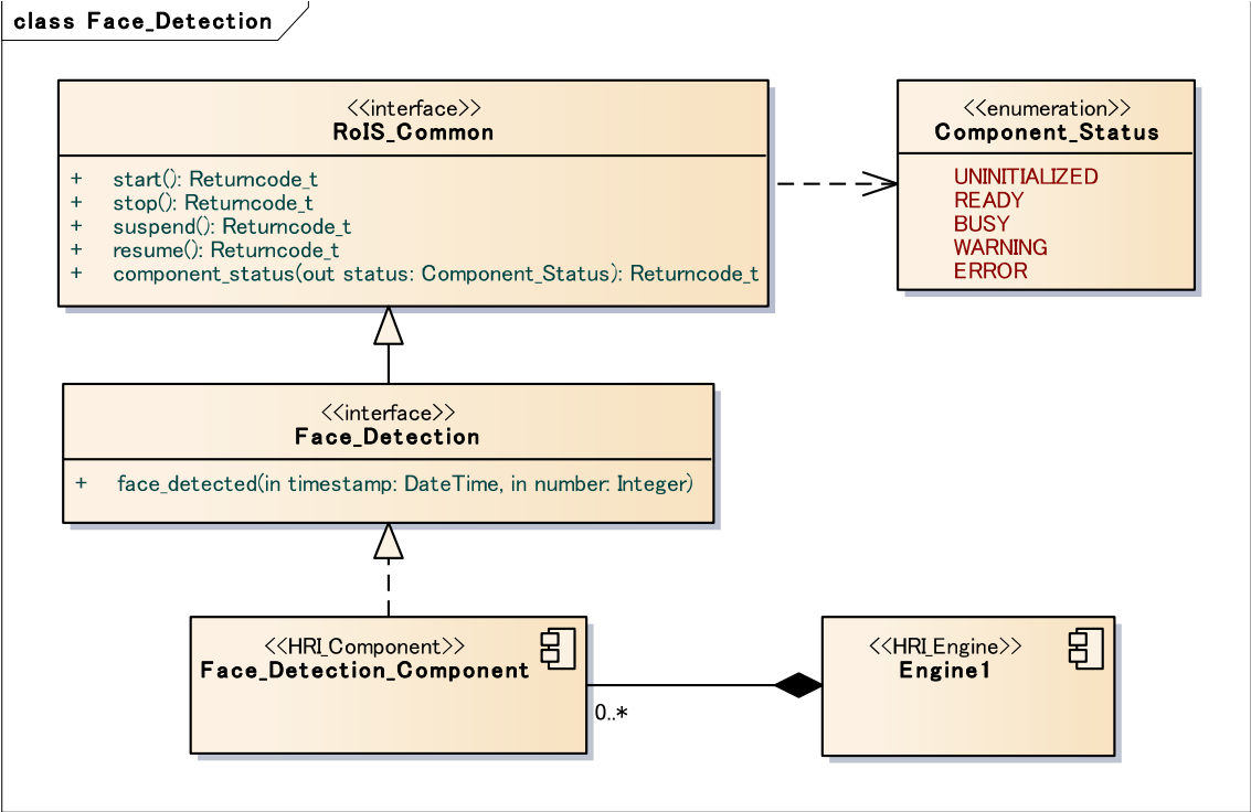
Figure 21 - face detection
