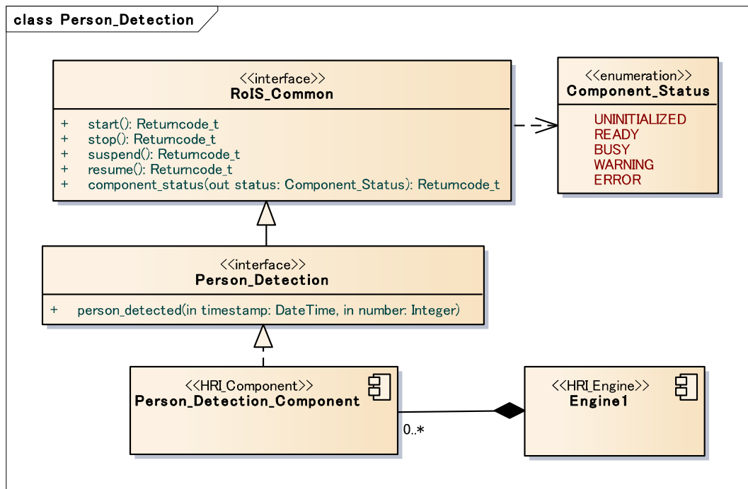
Figure 18 - person detection
