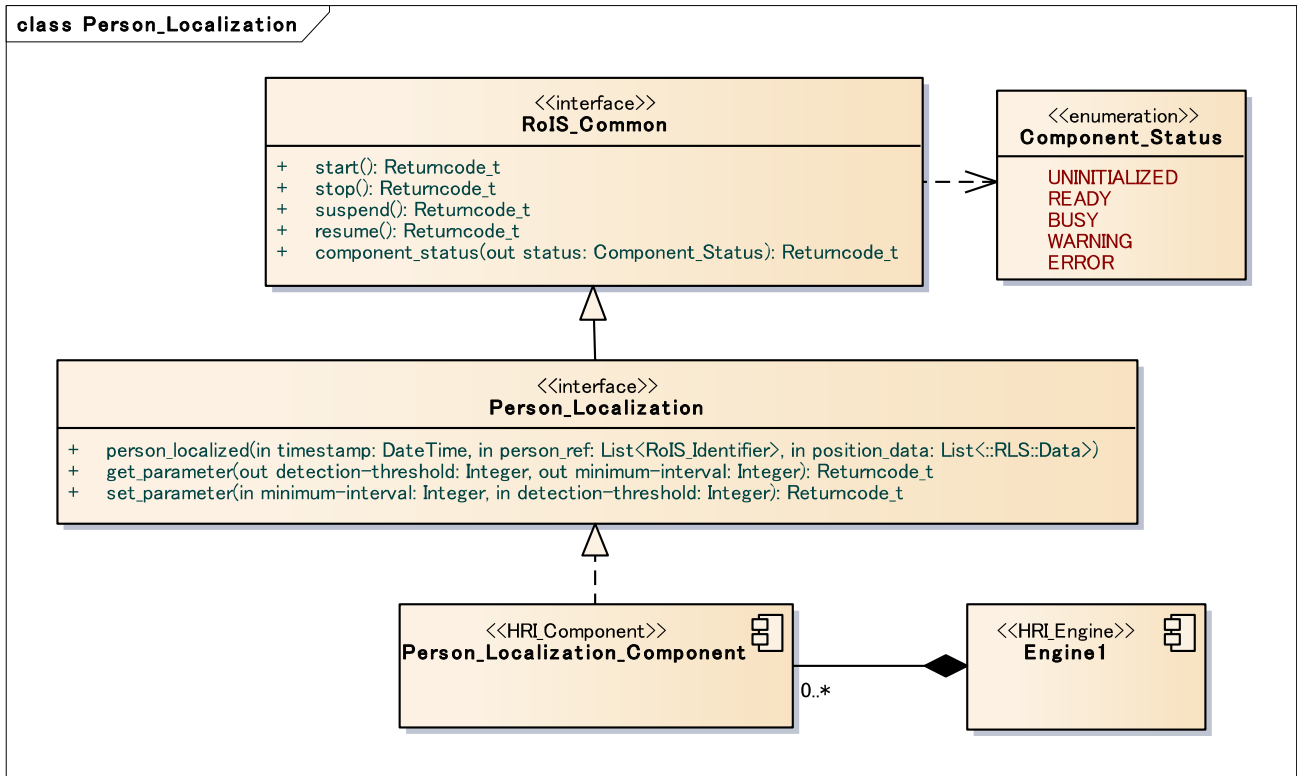
Figure 19 - person localization
