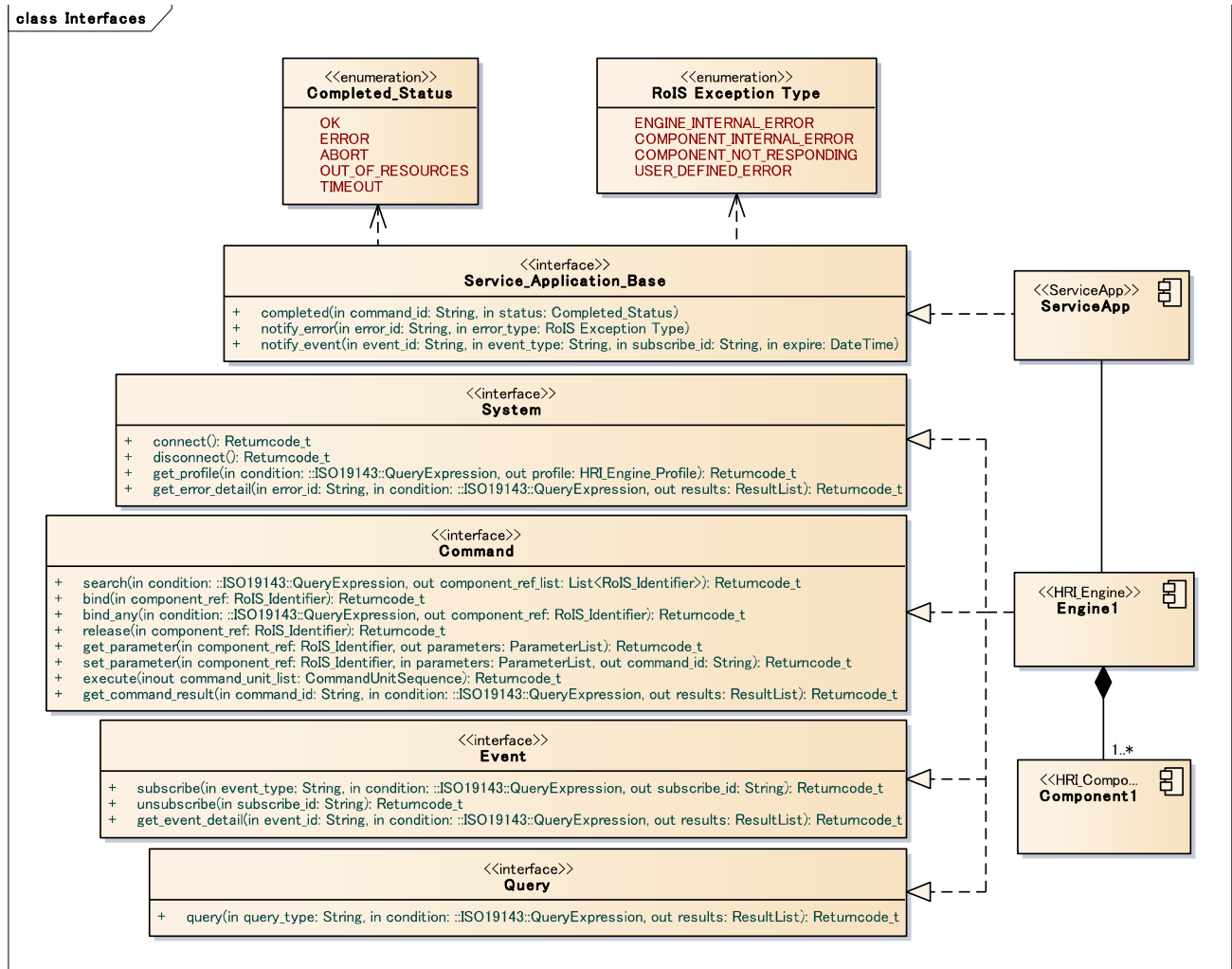
Figure 14 - RoIS Interfaces
