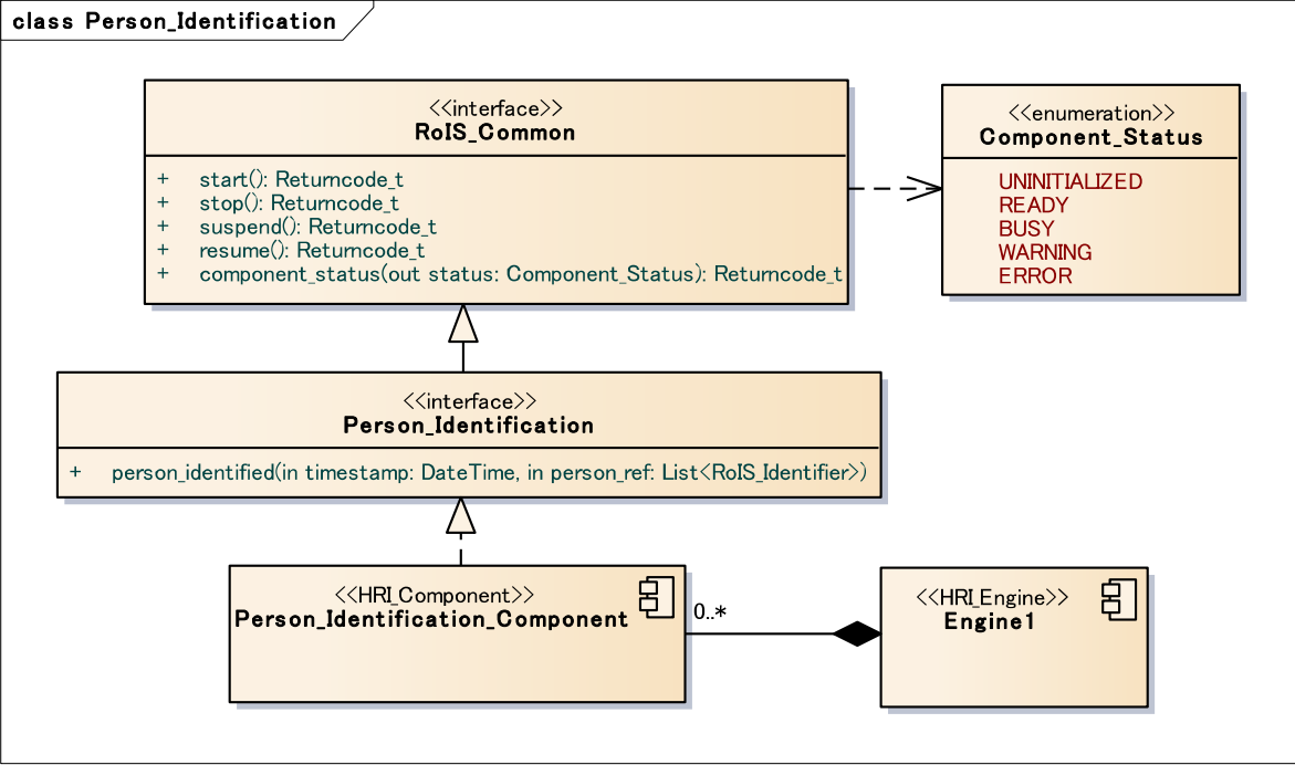
Figure 20 - person identification
