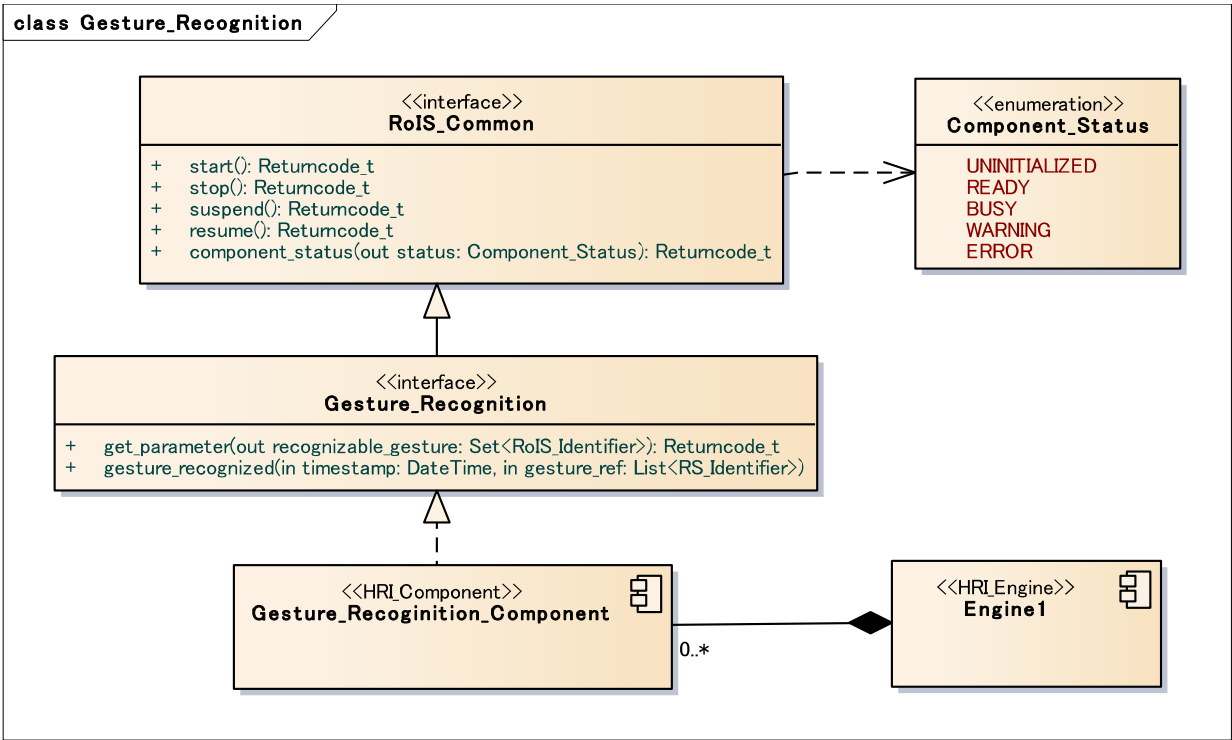
Figure 26 - gesture recognition
