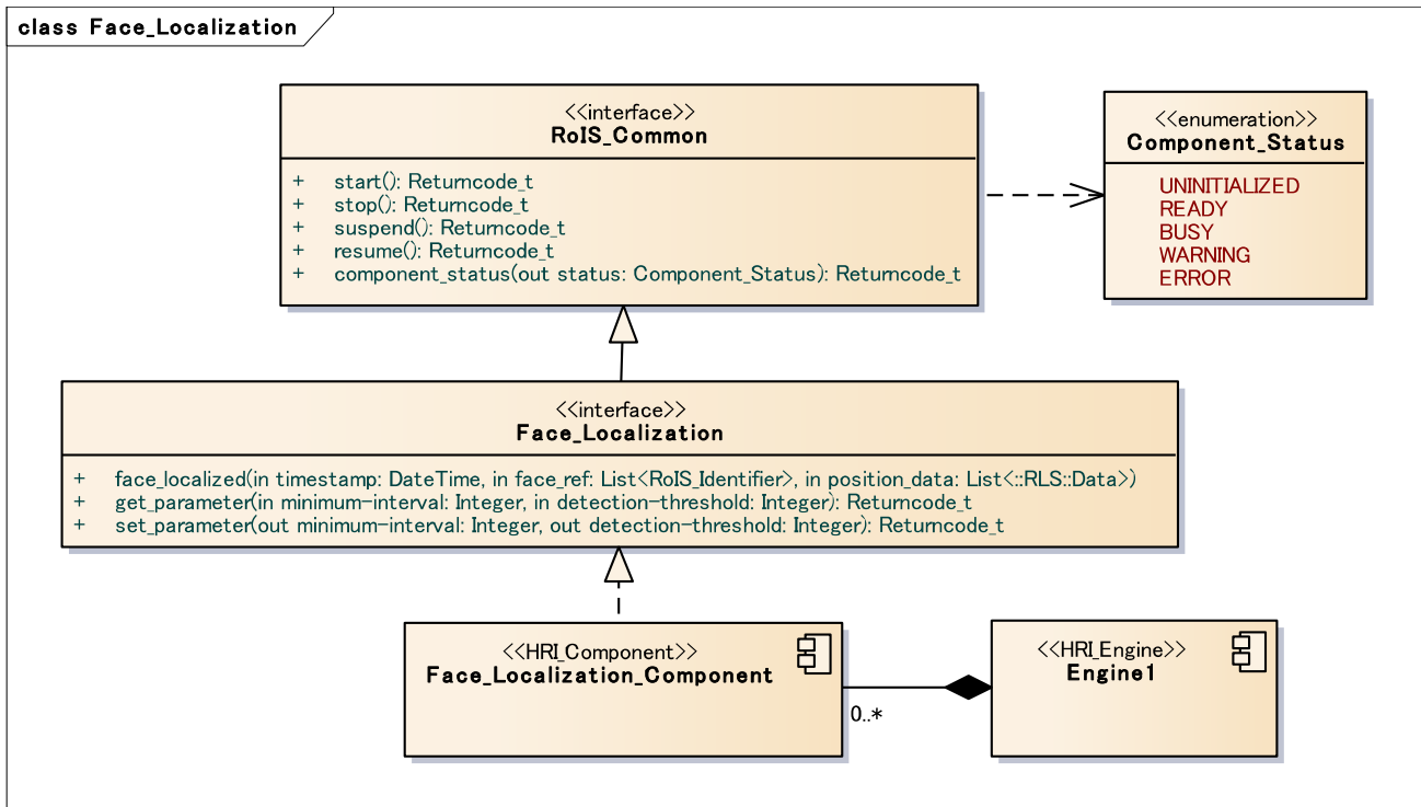
Figure 22 - face localization
