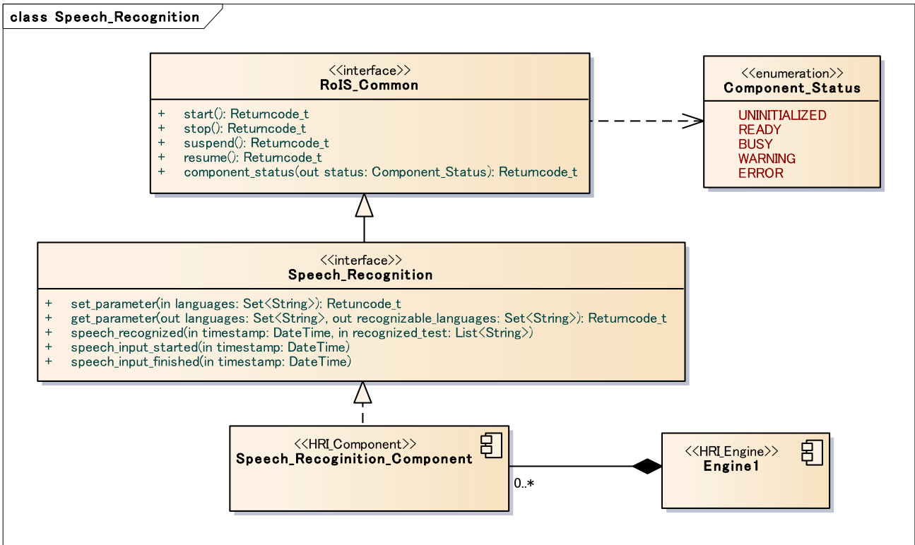
Figure 25 - speech recognition
