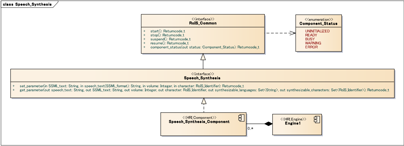
Figure 27 - speech synthesis
