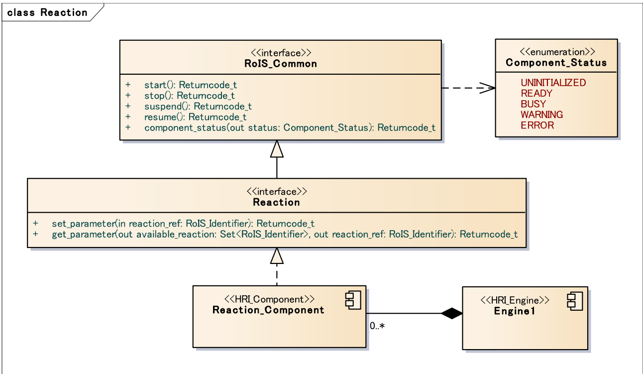
Figure 28 - reaction
