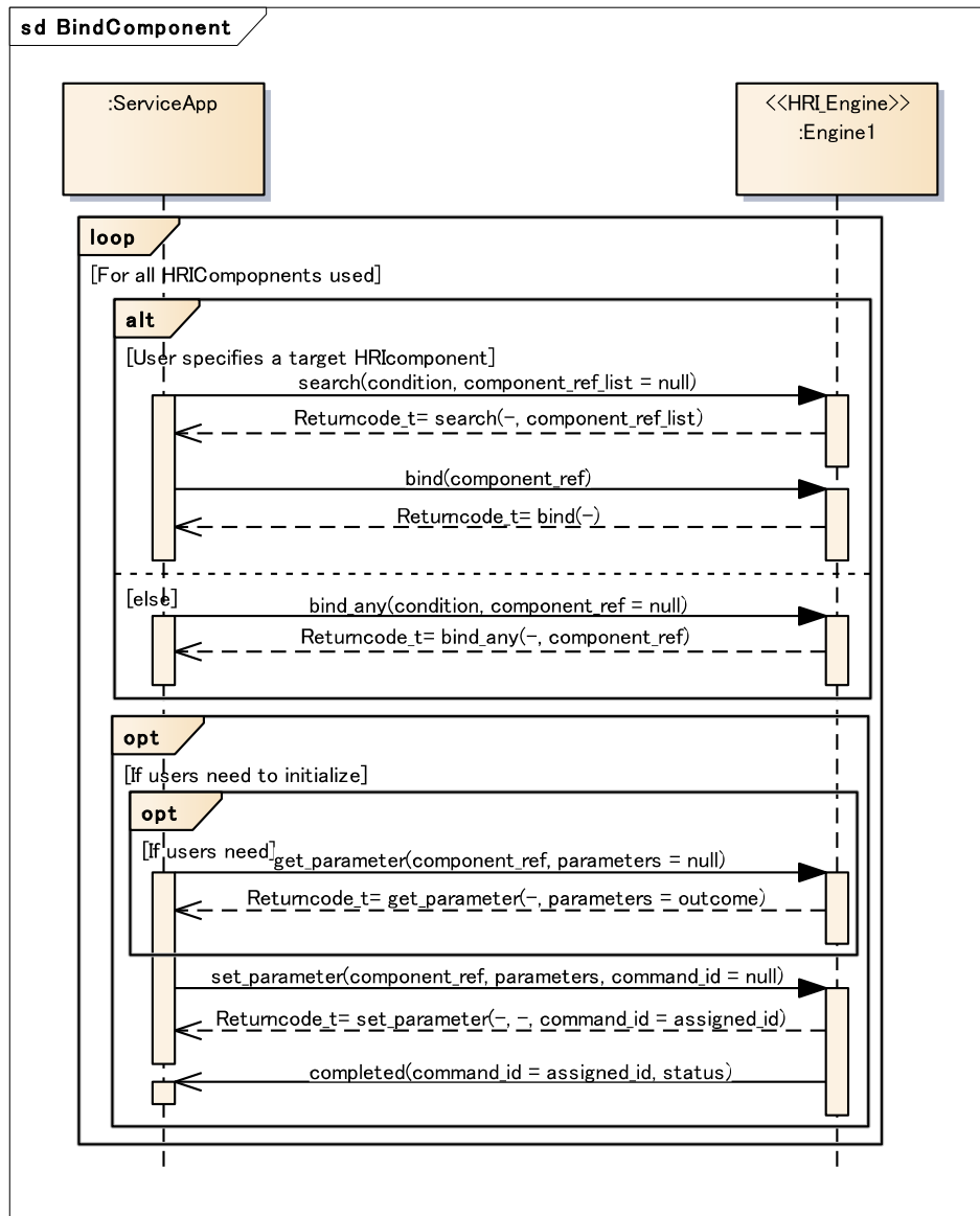
Figure 9 - Sequence Diagram of “BindComponent” in Command Interface
